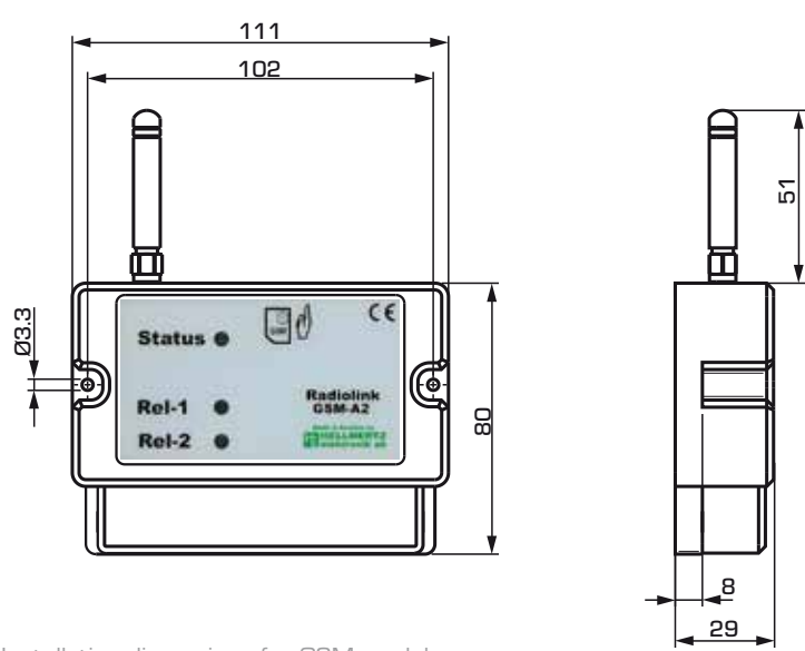
Installation dimensions for GSM module Series CRB915
