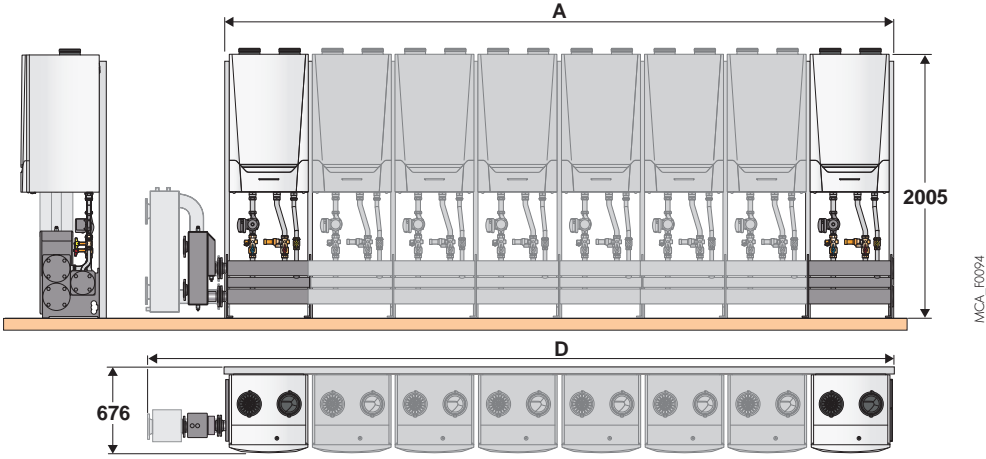
Floor-mounted alignment of 2 to 8 boilers
