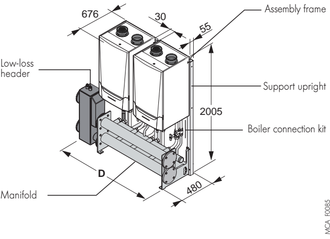
Floor-mounted alignment of 2 to 8 boilers
