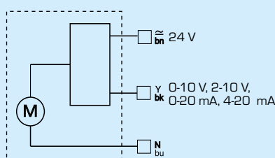
Actuator series ARA659
