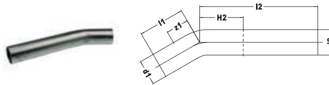
R2723 Bend tube 30° (2 x male)
