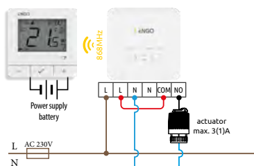
c) Wiring diagrams for the actuator
