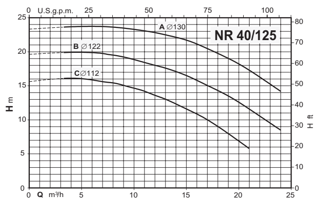
Coverage chart n \approx 2900 rpm
