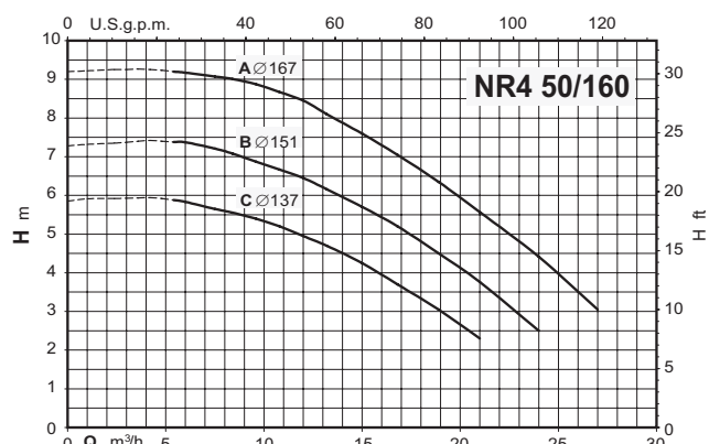
Coverage chart n \approx 1450 rpm
