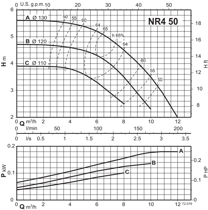
Coverage chart n ≈ 1450 rpm
