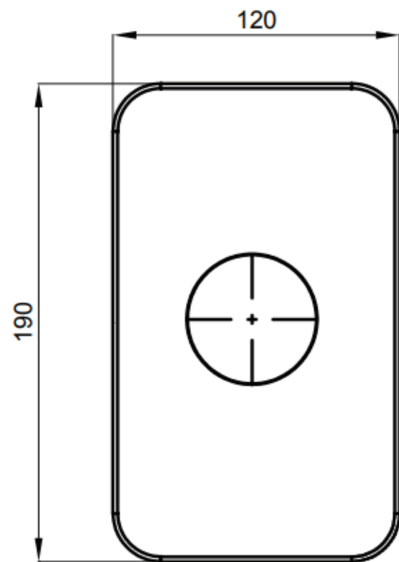
UH12249 chromium
